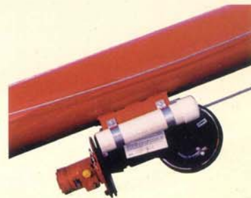
Hydraulic motor powers the worm winch lift, lifting and lowering at a smooth, steady pace.
